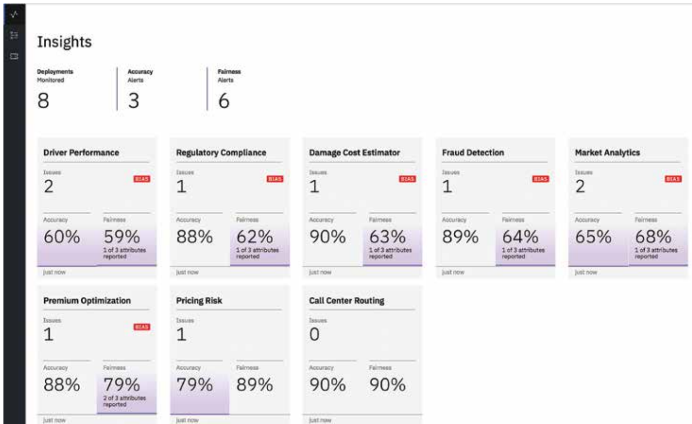
Figure A: Track AI application health in real-time to assess accuracy, fairness, and performance
